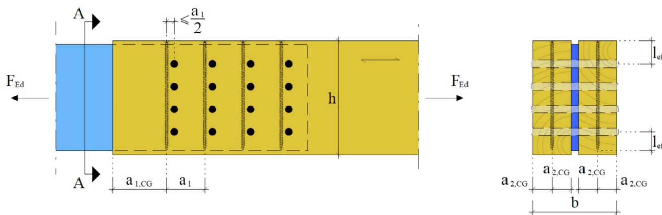
Figure A.4.3 Dowelled steel-to-timber connection with outer timber members and reinforcement
