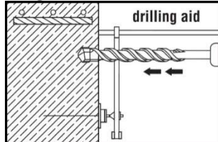
Figure B2: Example of drilling aid
