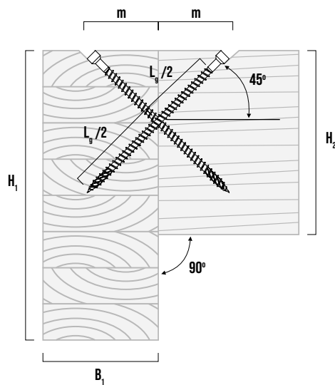
Cross-section
